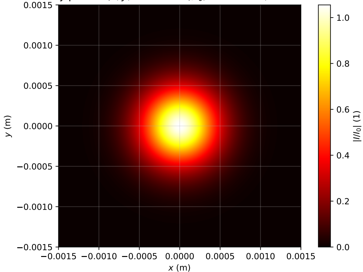
Intensity profile I(x, y, z = 0.637m)/I_0 , Pin=0.5Pcr, artificial time
